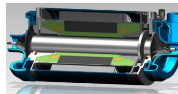
Electric Subsystems
