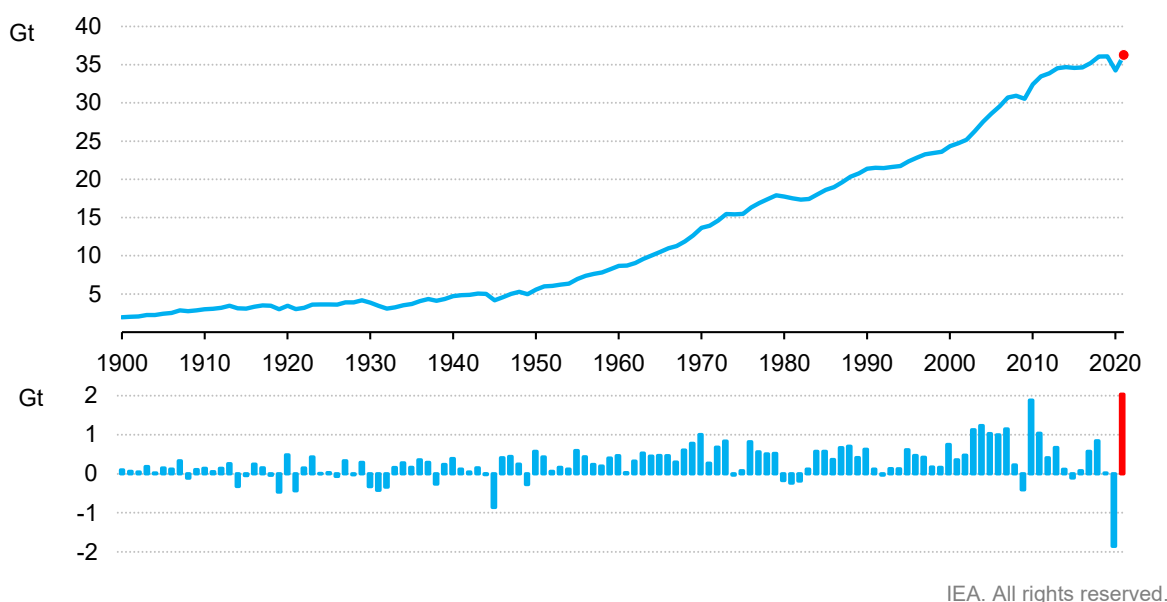
Figure 1 Total CO 2 emissions from energy combustion and industrial processes and their annual change, 1900-2021
